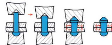
Cold-riveting
