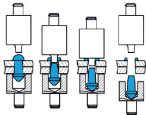
De-riveting
